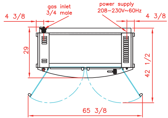
Top view Rotisserie with roof
